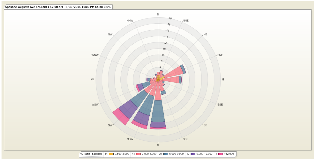
Figure 3: The wind rose depicts the variation of hourly average wind speed (mph) with the direction from which the wind was blowing in June.
