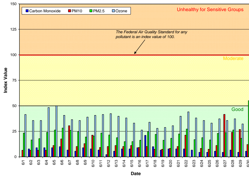
Figure 1: Air Quality Index (AQI) values for June 2011
