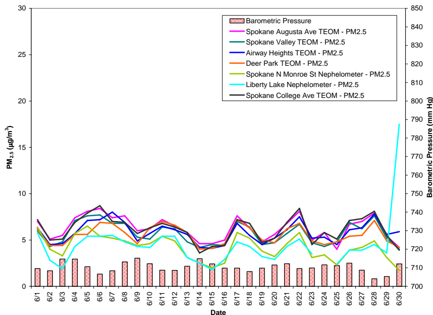
Figure 2: PM 2.5 multi-station time series for June 2011
