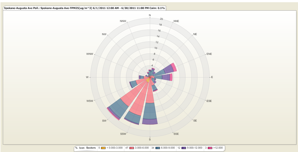
Figure 4: The PM 2.5 pollution rose depicts the variation of hourly average PM 2.5 ( \mu\text{g}/\text{m}^3 ) with the direction from which the wind was blowing in June.
