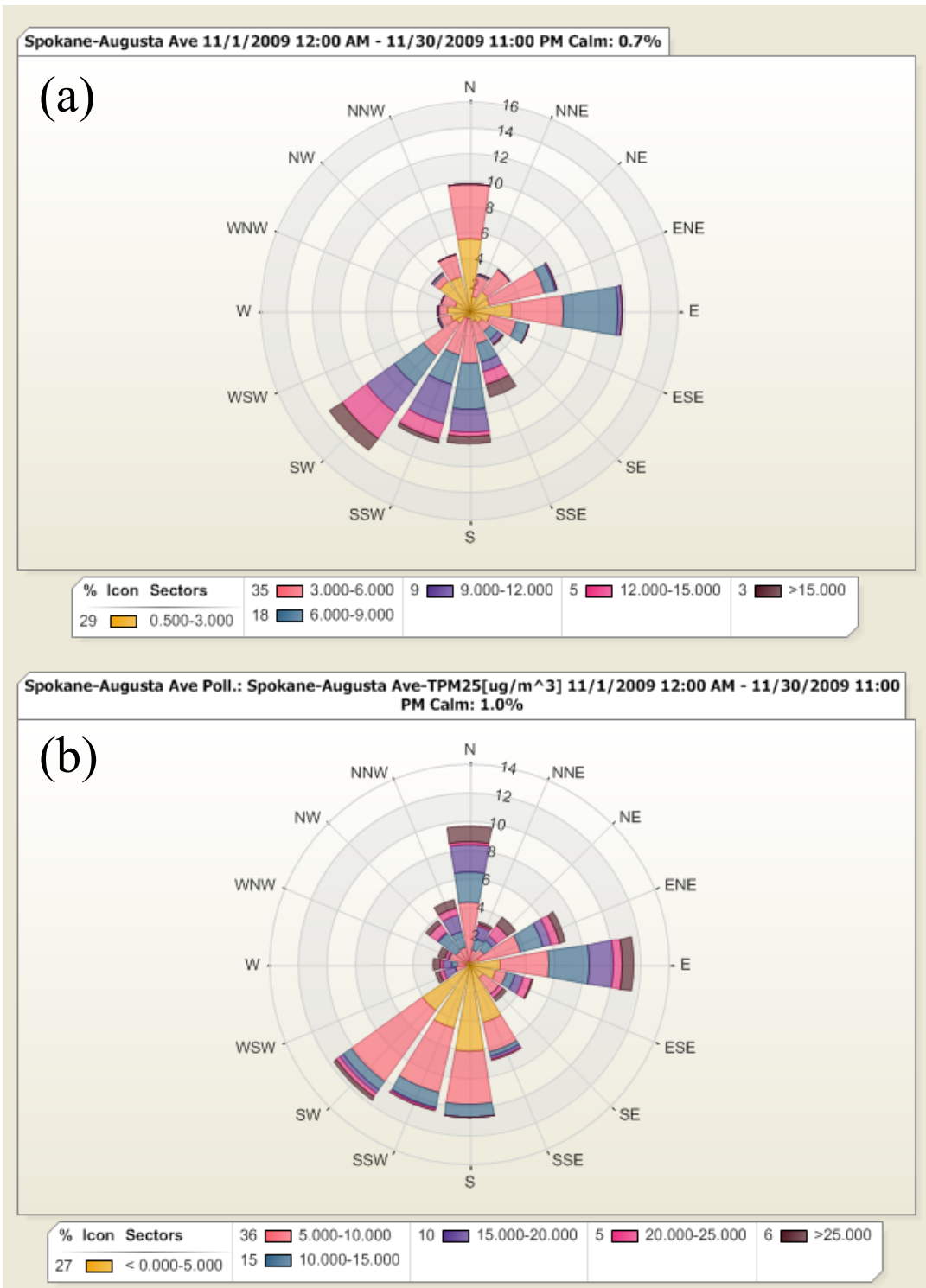
Figure 3: The wind rose (a) and PM 2.5 pollution rose (b) summarize the percentage of time during the month of November that wind speed and PM 2.5 , respectively, varied with wind direction. The charts are derived from hourly-averaged data.
