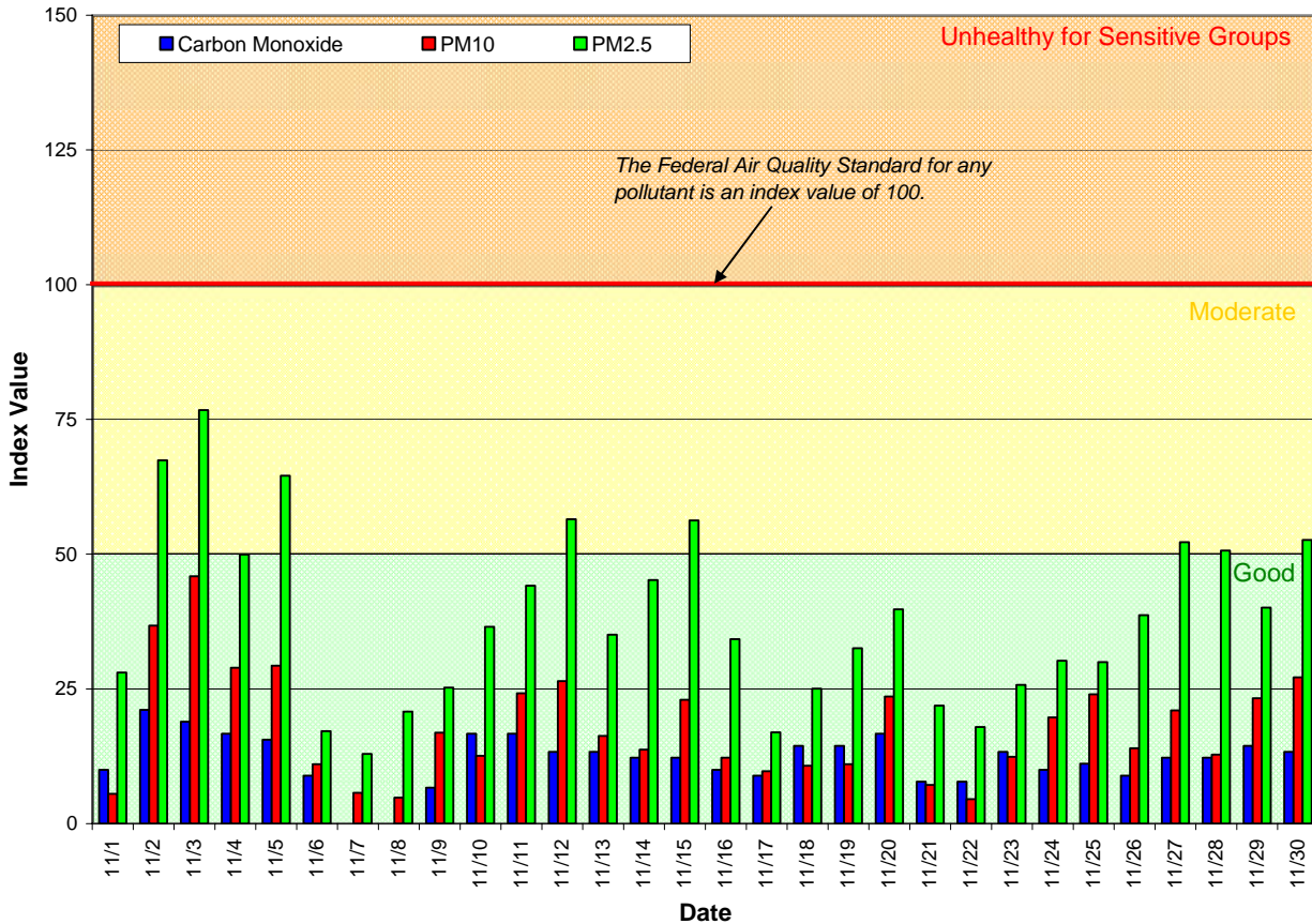
Figure 1: Air Quality Index (AQI) values for November 2009
