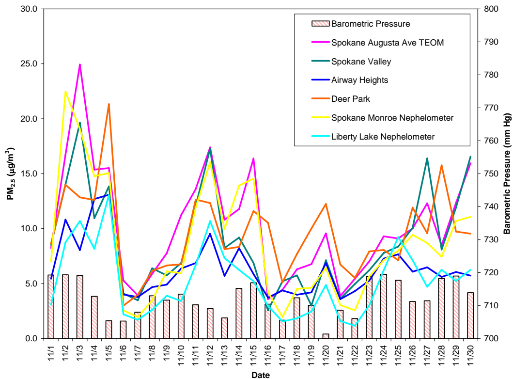
Figure 2: PM 2.5 multi-station time series for November 2009
