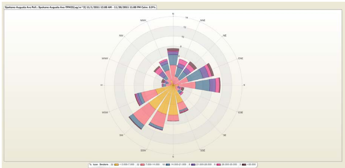
Figure 4: The PM 2.5 pollution rose depicts the variation of hourly average PM 2.5 (µg/m 3 ) with the direction from which the wind was blowing in November.
