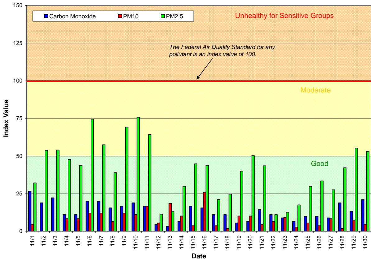
Figure 1: Air Quality Index (AQI) values for November 2011
