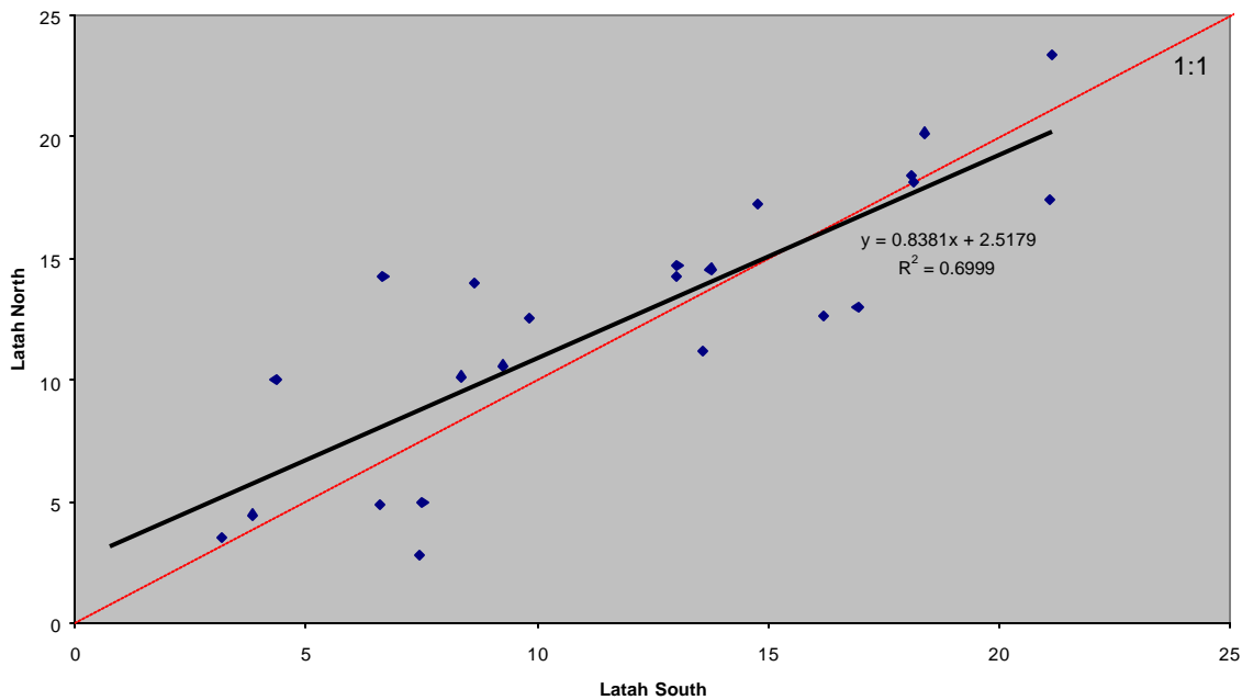
Figure 16: Spokane, Washington Ambient PM 2.5 Concentrations (mg m -3 ) Latah N v. Latah S PM 2.5 5/99 - 11/99
